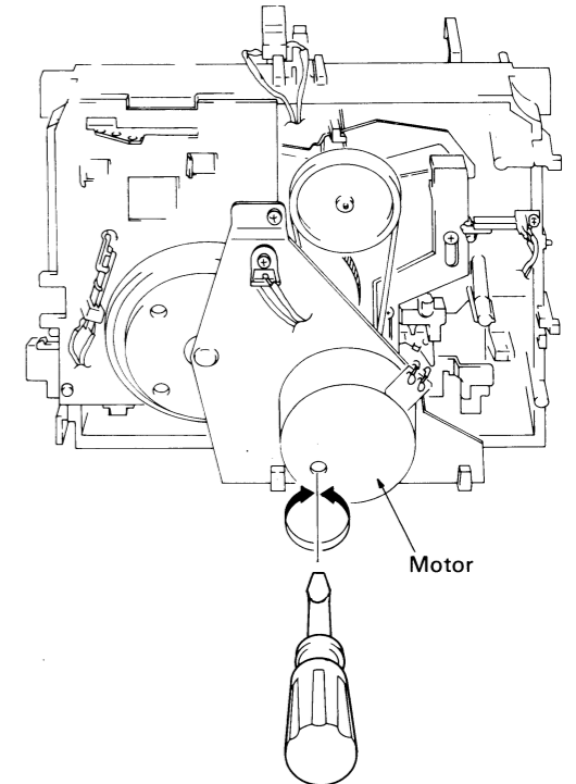
Fig. 11-2 Arrangement diagram of adjusting parts
